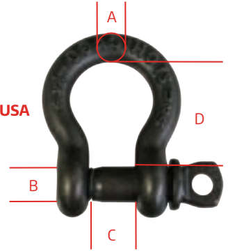
THSPA500BL
