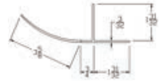
HS-22S
