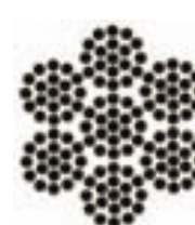
7 x 19 - EXTRA FLEXIBLE
