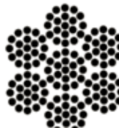
7 x 19 - EXTRA FLEXIBLE
